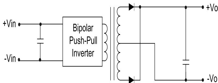
Single Output Block Diagram
