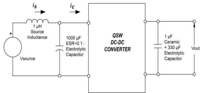
Fig. 2: Test setup for measuring input reflected ripple currents i_c
