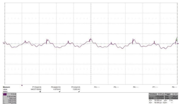
Fig. 13: Input reflected ripple current, i_c (500 mA/mV), measured at input terminals at full rated load current at V_{IN} = 24V . Refer to Fig. 2 for test setup. Time: 2 \mu s/div. RMS input ripple current is 1.205 \times 500mA = 602.5mA .
