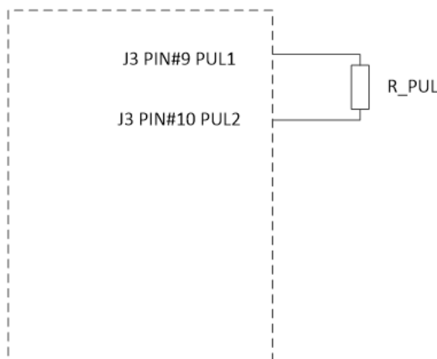
External resistor connection for PUL
