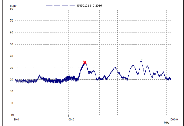
Radiated Emission Test, (110Vin, 12V @ 24A out)
