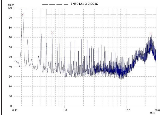
Conducted Emission Test, (110Vin, 12V @ 24A out)
