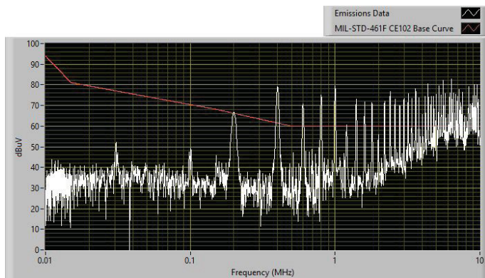
a) Without input filter. CIN = 2 x 470µF/50V/70mΩ.
