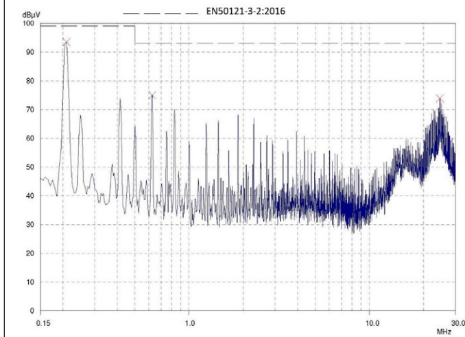
Conducted Emission Test, (110Vin, 12V @ 24A out)
