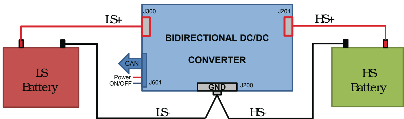
The 48S12.3K0BCA block diagram.
