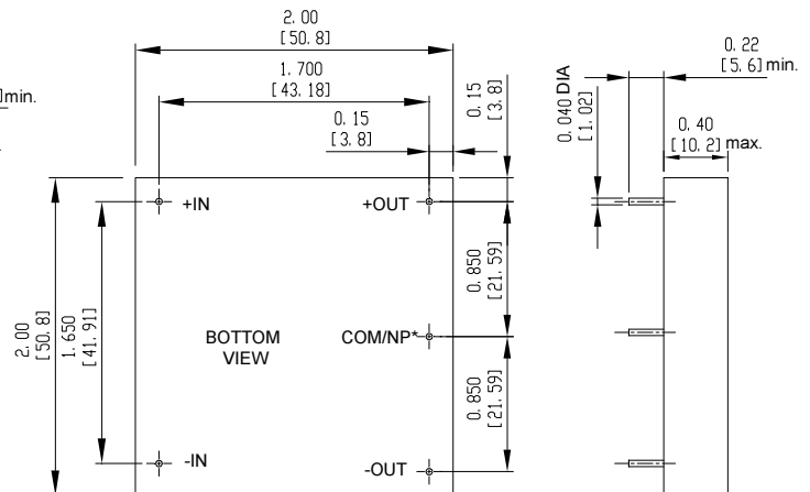
ALTERNATE PIN CONFIGURATION SUFFIX "S"
