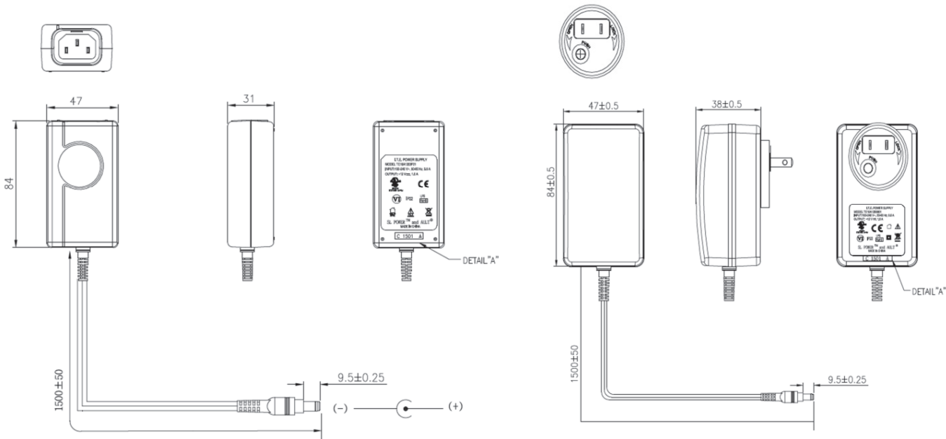
Interchangeable N.A. Blade, 2.5mm x 5.5mm x 9.5mm Barrel Connector
