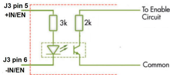
XgA-XgD Remote Enable/Disable of Output
