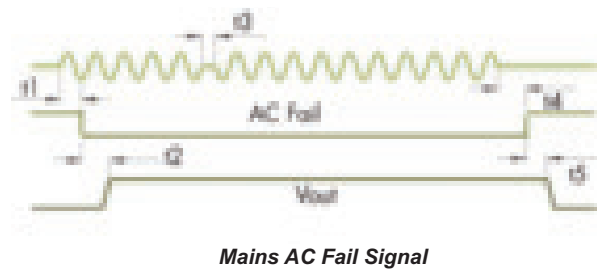
Mains AC Fail Signal
