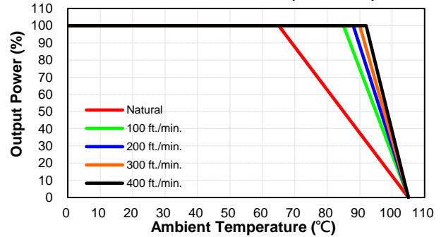
CQB75-300S12, 15, 24, 48 Derating Curve with Heatsink QBT210 (Vin=300V)
