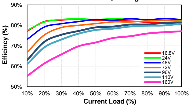
CQB50W12-72S05-CMFC Eff Vs Io @25 Deg. C
