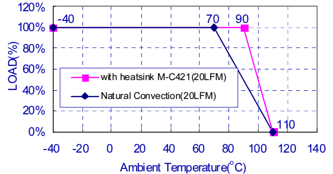
Typical Derating Curve
