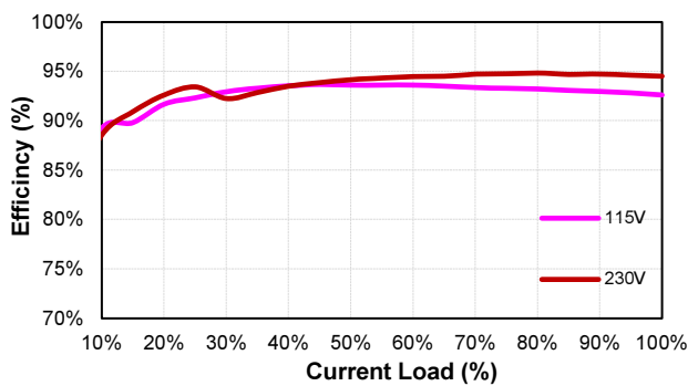
CFM500M240 (Eff Vs Io)
