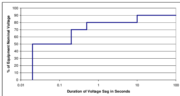
Figure 2 Recommended Voltage Sag Immunity
