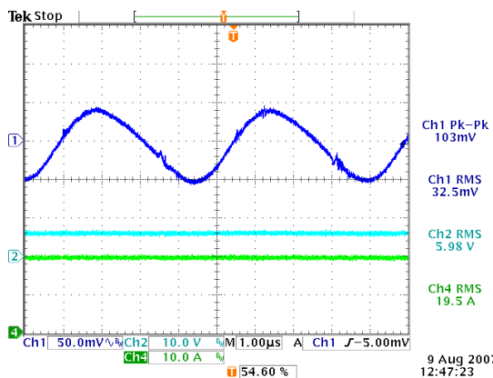
Fig X: Ripple and Noise measured on an Xg3 under full load conditions Ambient = +50°C
