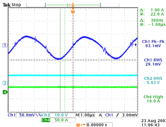
Fig X: Ripple and Noise measured on an Xg3 under full load conditions Ambient = -20°C
